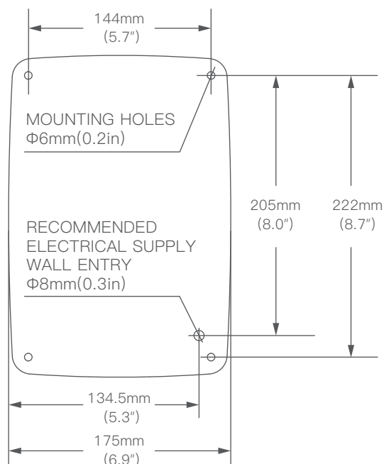
FRONT VIEW FACING WALL
